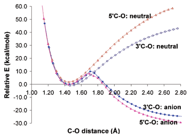
Figure 2. Adiabatic potential energy surfaces for 3'C–O and 5'C–O bond rupture. All energies are relative to the energies of the anions at equilibrium.
