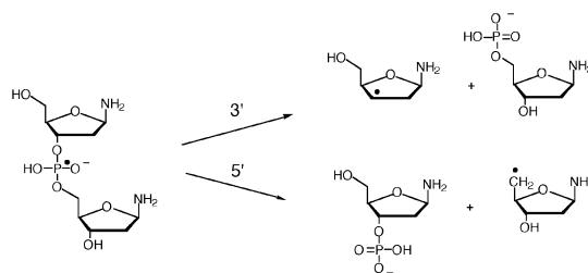
Figure 1. Sugar–phosphate–sugar model representing a section of DNA backbone. Electron-induced bond dissociations at the 3' and 5' ends of the model are investigated.
